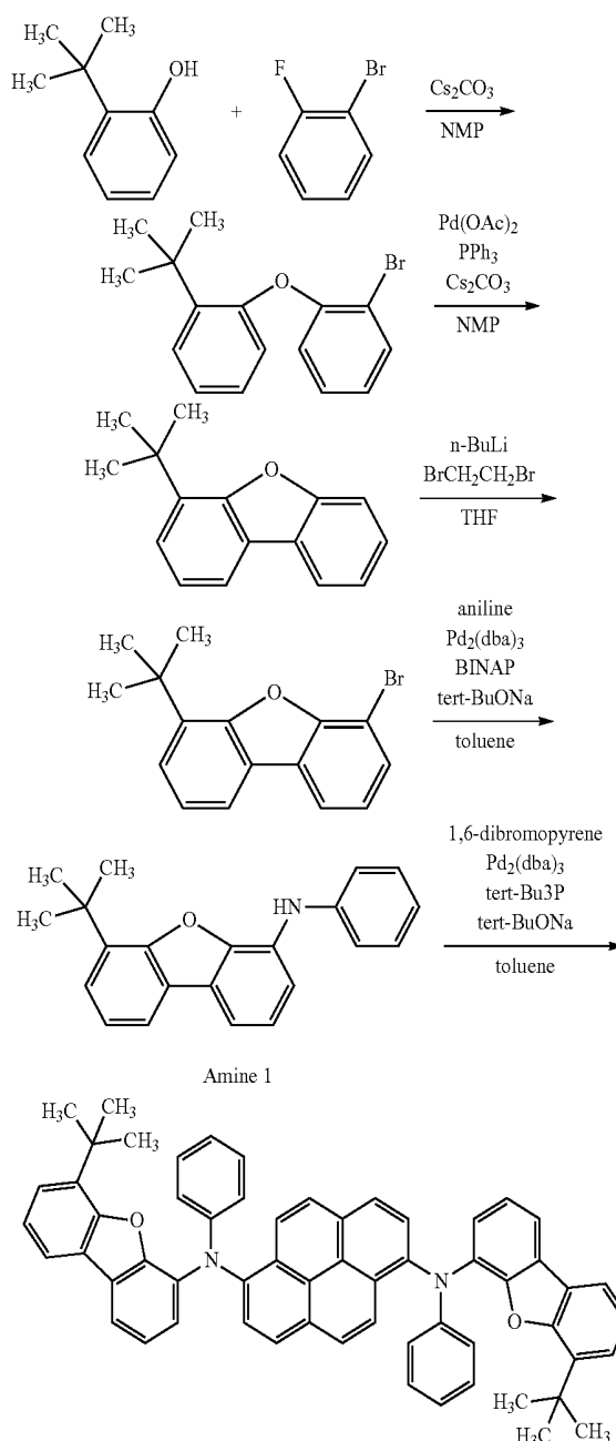
Compound 1
