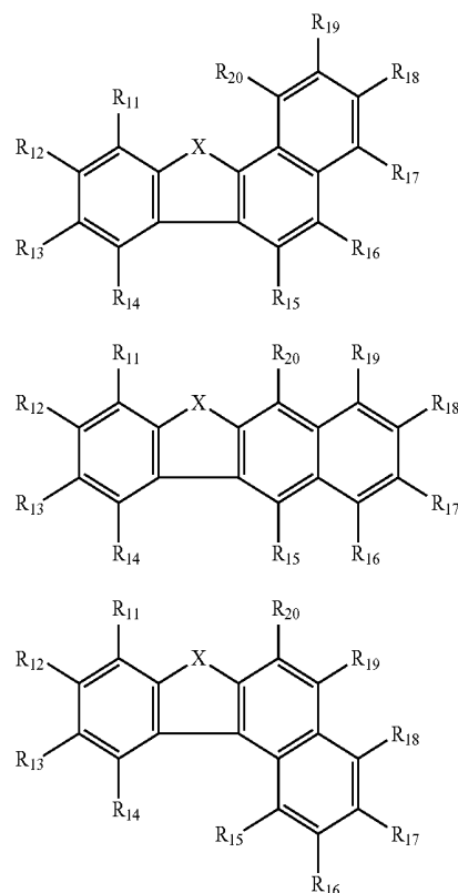
[Formula 6]
