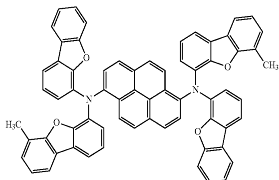
Compound 9
