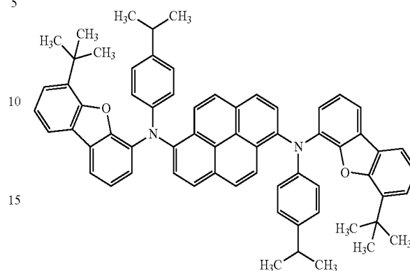
Compound 4
