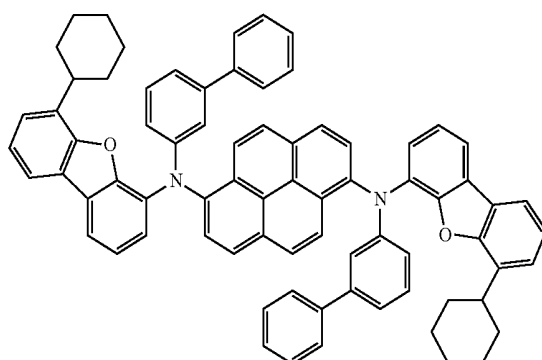
Compound 8
