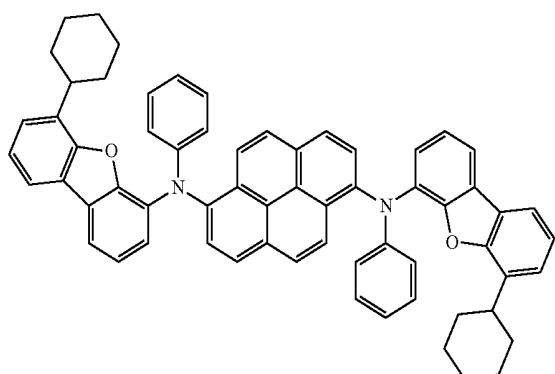
Compound 6
