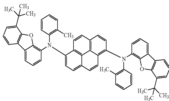
Compound 7
