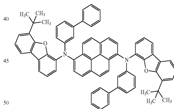
Compound 5
